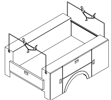
Bow Ladder Rack
